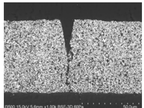
Pre-cut Argomax film allows for more accurate Argomax placement onto the die or spacer. The material is pre-cut to enable more consistent release from the backer/carrier film.
