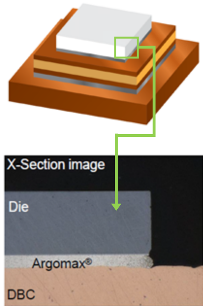
Argomax attached to die and DBC before sintering to show Argomax placement accuracy with AccuLam.
